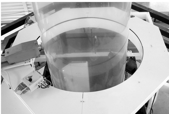
Contact / Non-Contact Capacitive sensor with Telescopic arm
